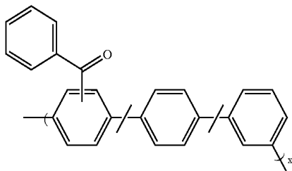
Poly(2,5-benzophenone-co-1,4-phenylene-co-1,3-phenylene), 25
